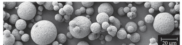
SEM image of SphereTEC® fillers
