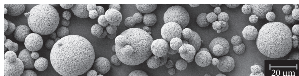
SEM image of SphereTEC® fillers
